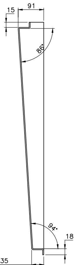
SECTION AA
